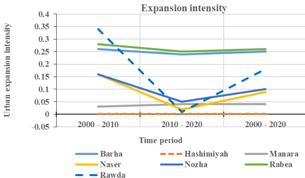
Figure 2. Urban expansion intensities of the seven districts
