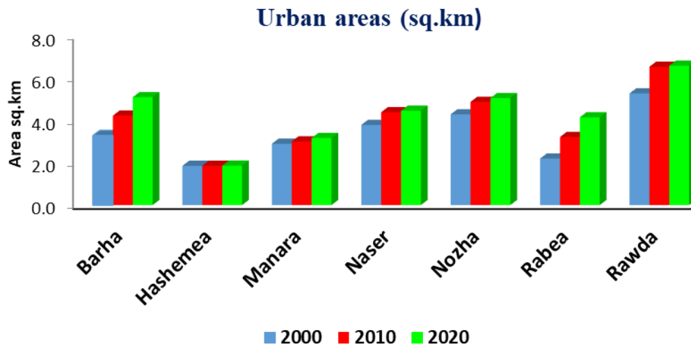
Figure 3. Urban areas ( \text{km}^2 ) included in the study
