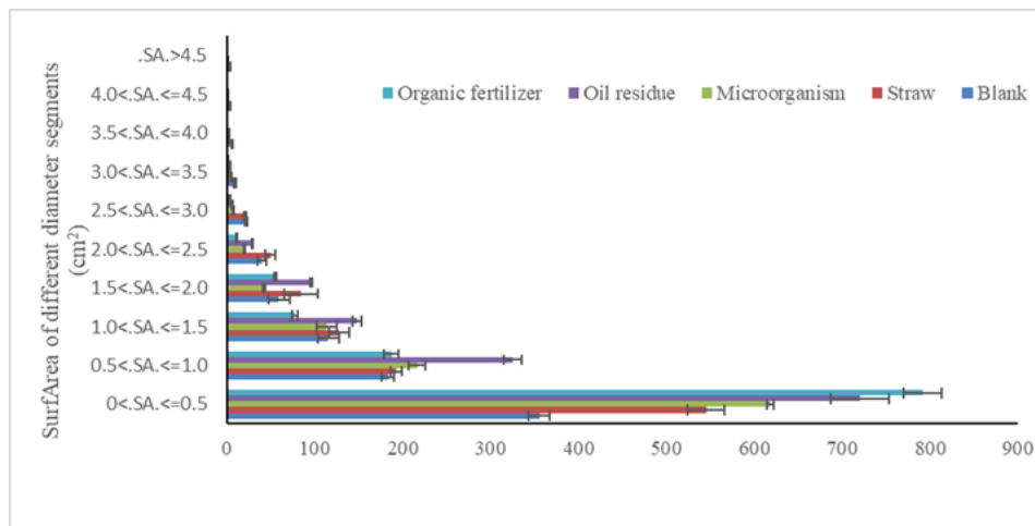
Figure 14. Root surface area in different root diameter regions
