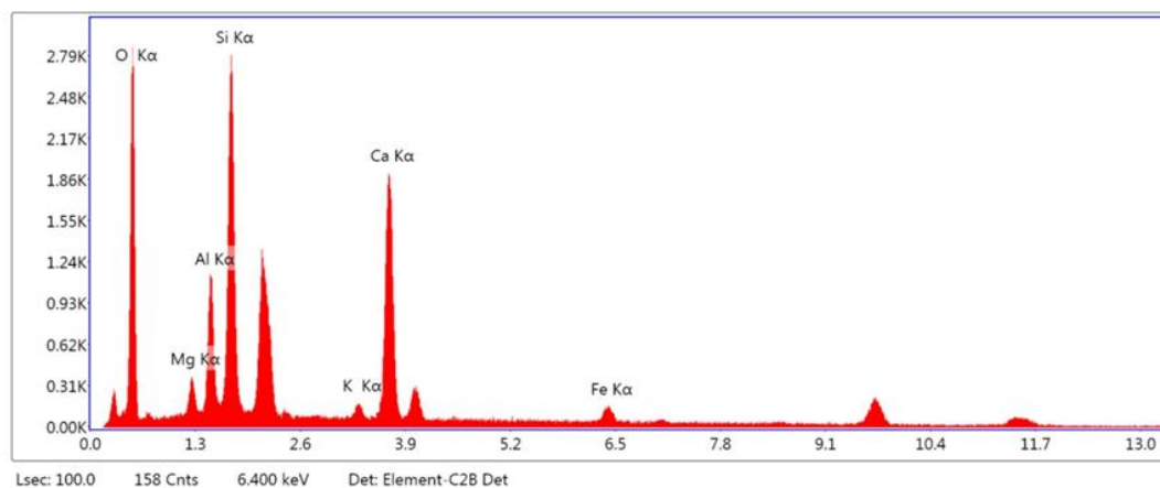
Figure 5. Energy spectrum of soft rock
