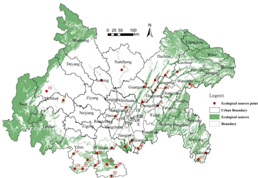
Figure 4. Spatial distribution of ecological source sites in the study area. (1-30: ecological source numbering, I.: Beibei, II.: Shapingba, III.: Bishan, IV.: Jiulongpo, V.: Dadukou, VI.: Yuzhong, VII.: Nan'an, VIII.: Jiangbei, IX.: Yubei, X.: Banan)
