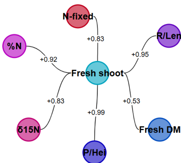
Figure 6. Fresh shoot vs plant height (plant height), shoot dry matter (fresh DM), root length (root length), \%\text{N} , \delta^{15}\text{N} , \text{N-fixed} . The correlation coefficient is the value that exists between two strong parameters that are significance at P < 0.05 , P < 0.01 , P < 0.001
